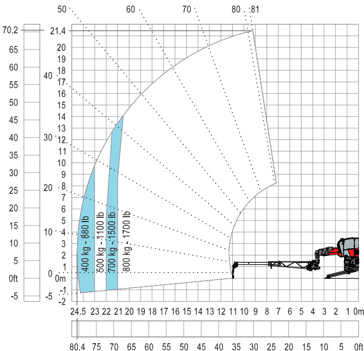
Potence-treuil extensible 800 kg
