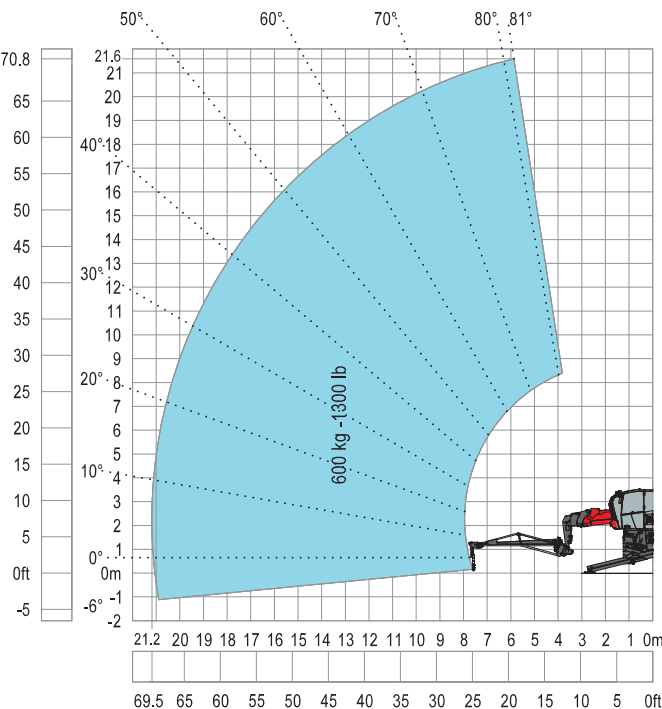
Potence-treuil 600 kg
